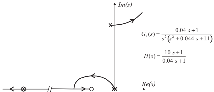
Figure 6.5: Two-mass problem, root locus plot for the non-collocated control with a lead compensator.
